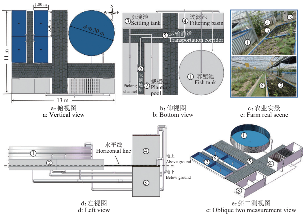
图 1 农场试验区种养单元示意图 Fig. 1 Schematic diagram of farming units in the farm trial area
